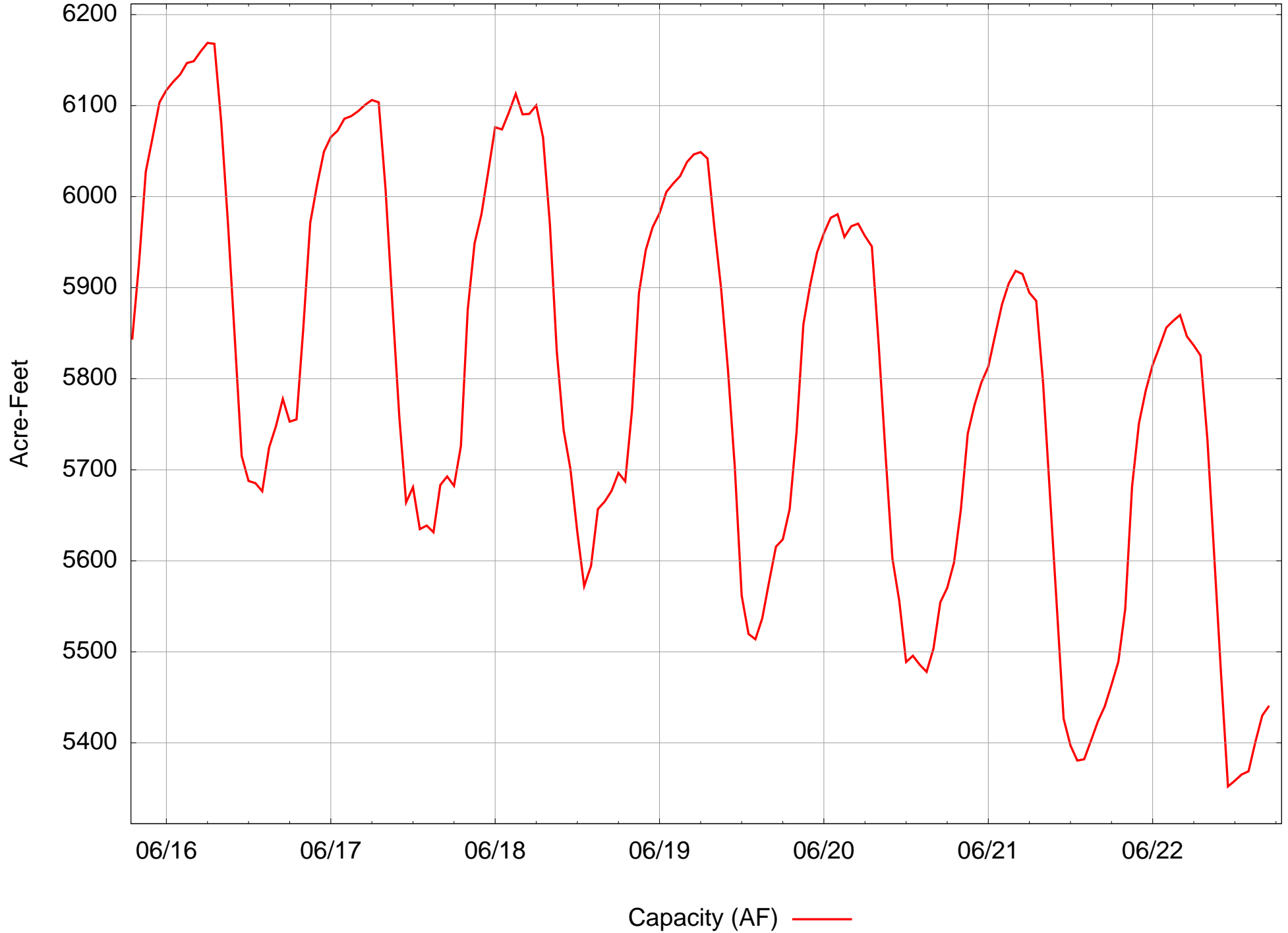
Minersville Reservoir Capacity
