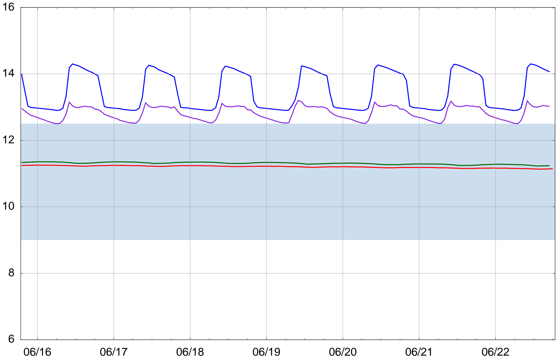
Rocky Ford Irrigation Hourly Average Battery Voltages
