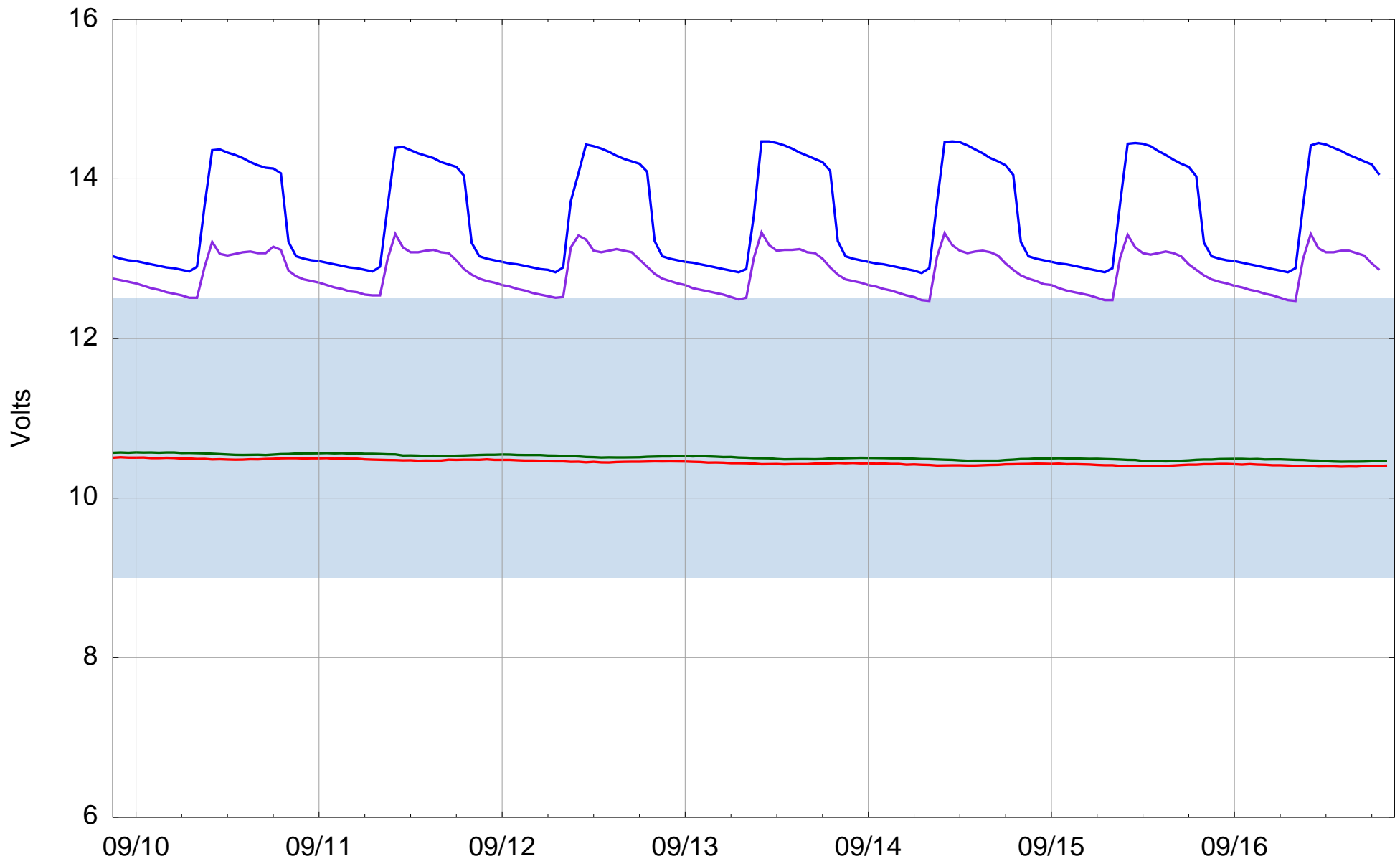
Rocky Ford Irrigation Hourly Average Battery Voltages
