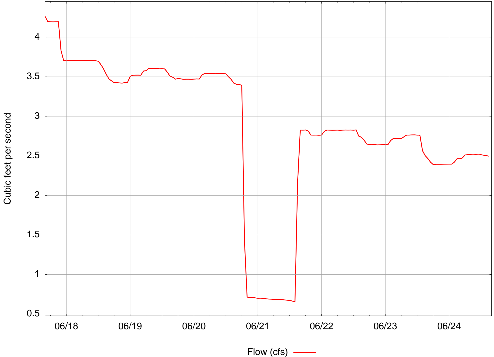
Lyon Parshall Flume Hourly Average Flow
