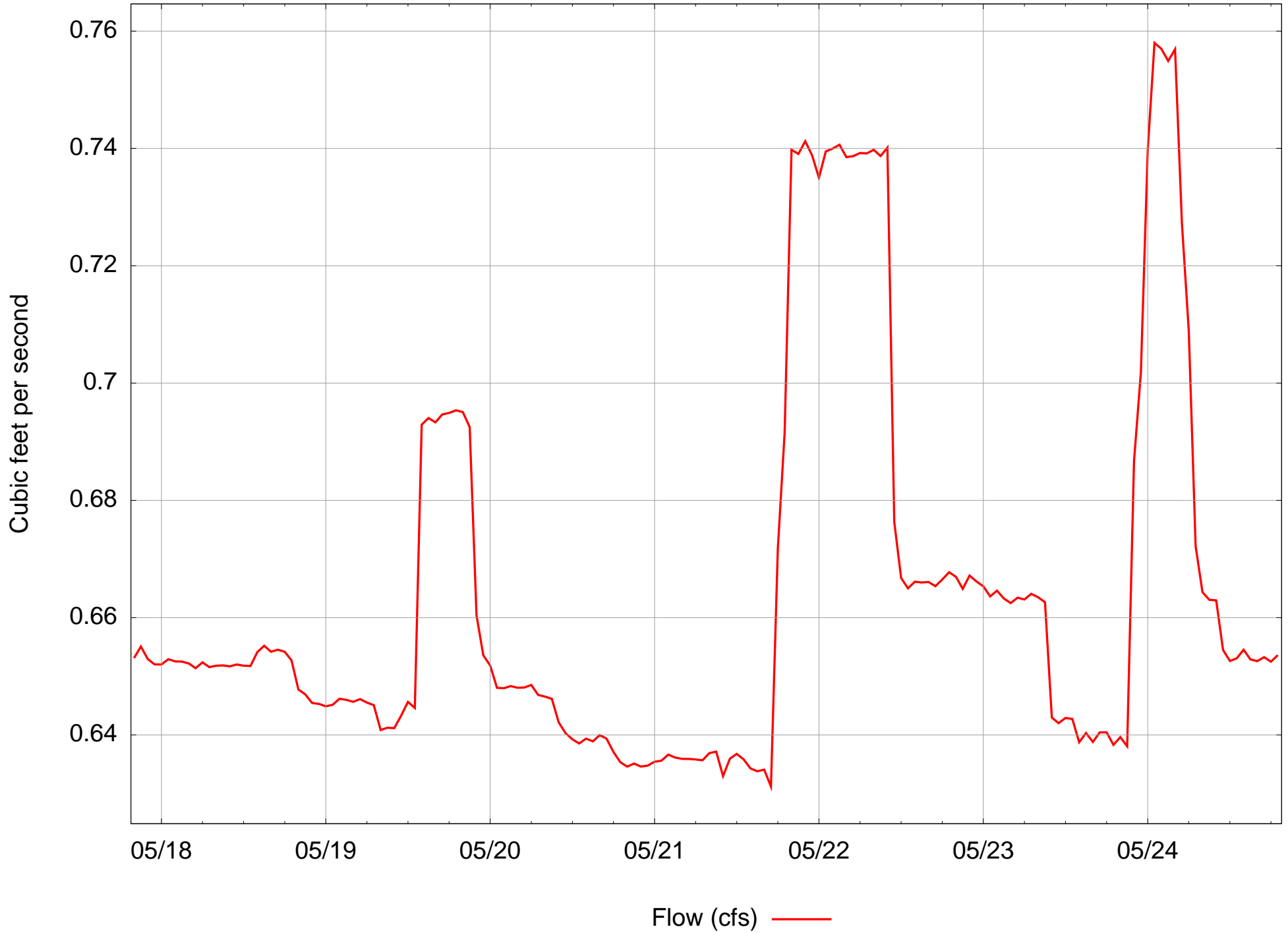
Taylor Parshall Flume Hourly Average Flow
