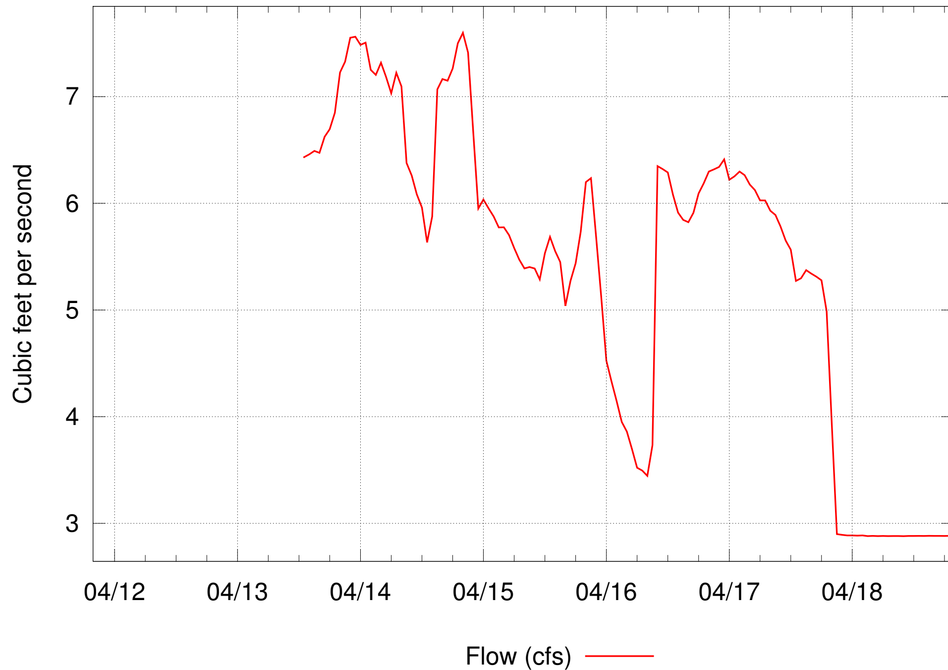
Acton Parshall Flume Hourly Average Flow
