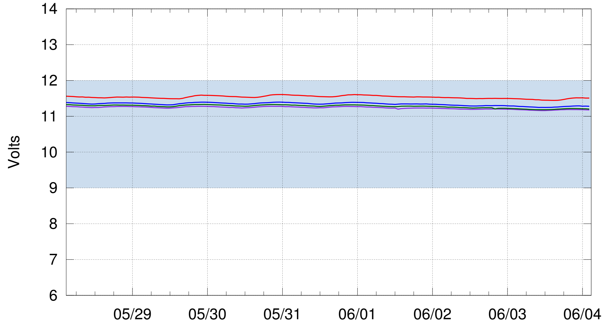
Hourly Average Battery Voltage
