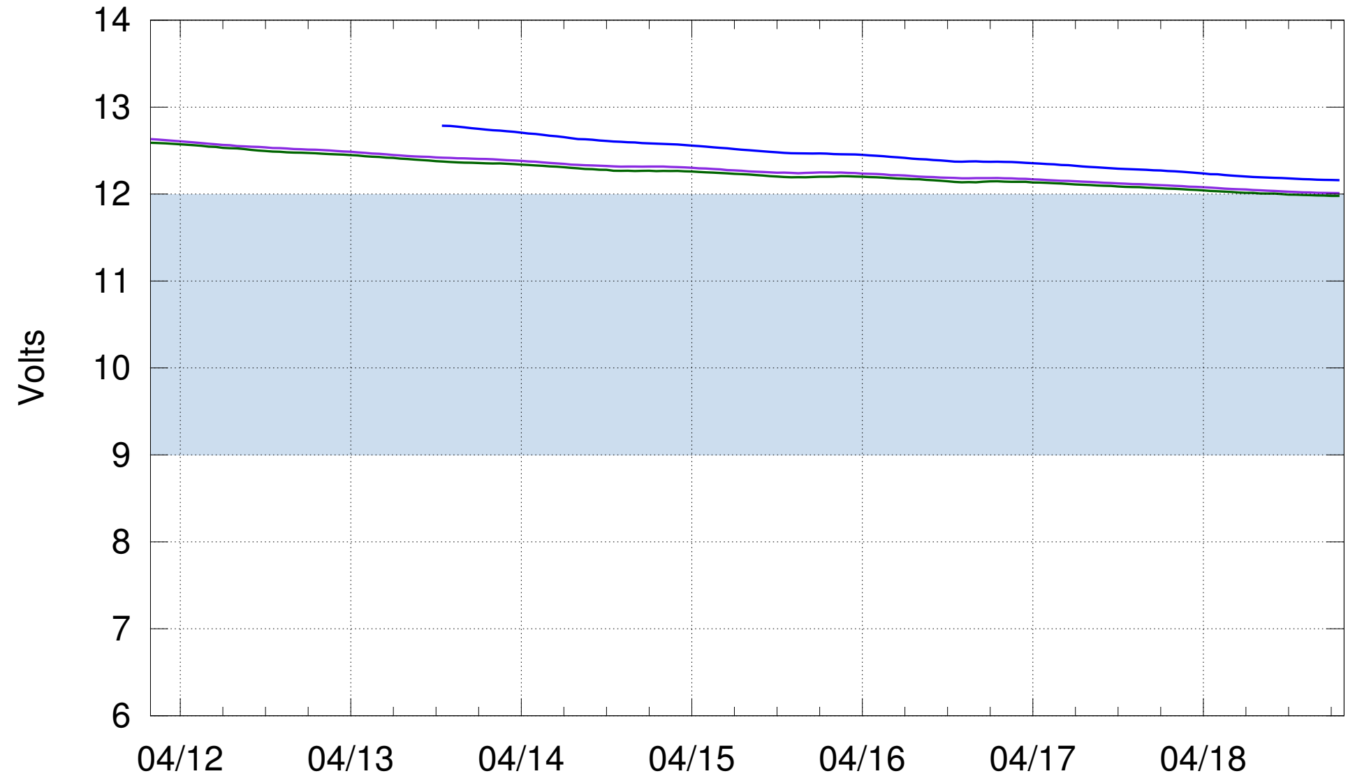
Hourly Average Battery Voltage
